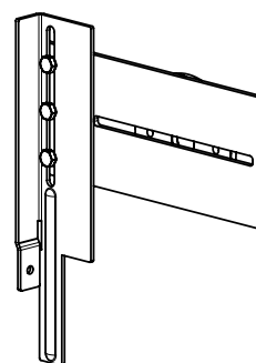
BEARING / MOTOR HOLDER – LEFT RVS 004 2-01349-XXX-1
