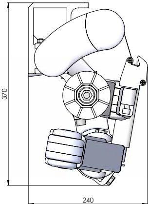
Console wall / ceiling – cross arms
